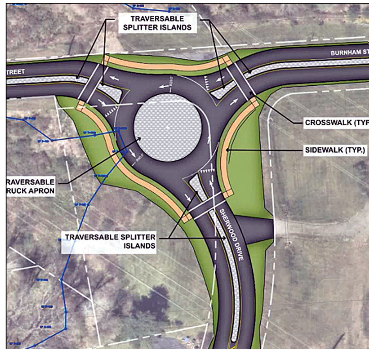
THE PLANNED BURNHAM AND SHERWOOD DRIVE ROUNDABOUT.
